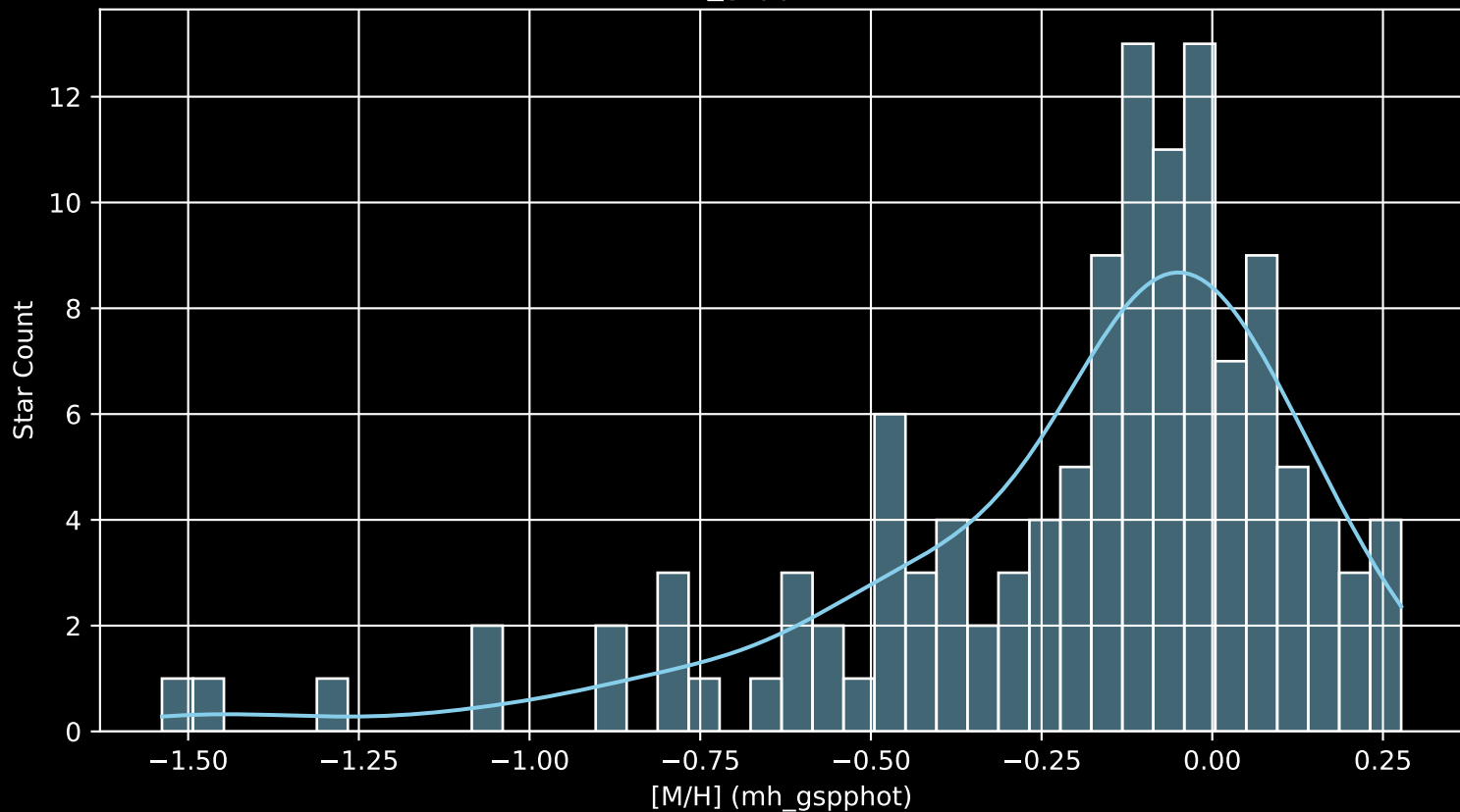
APOGEE DR17 Field: [317-12 [M/H] (mh_gspphot) (n= 123)
