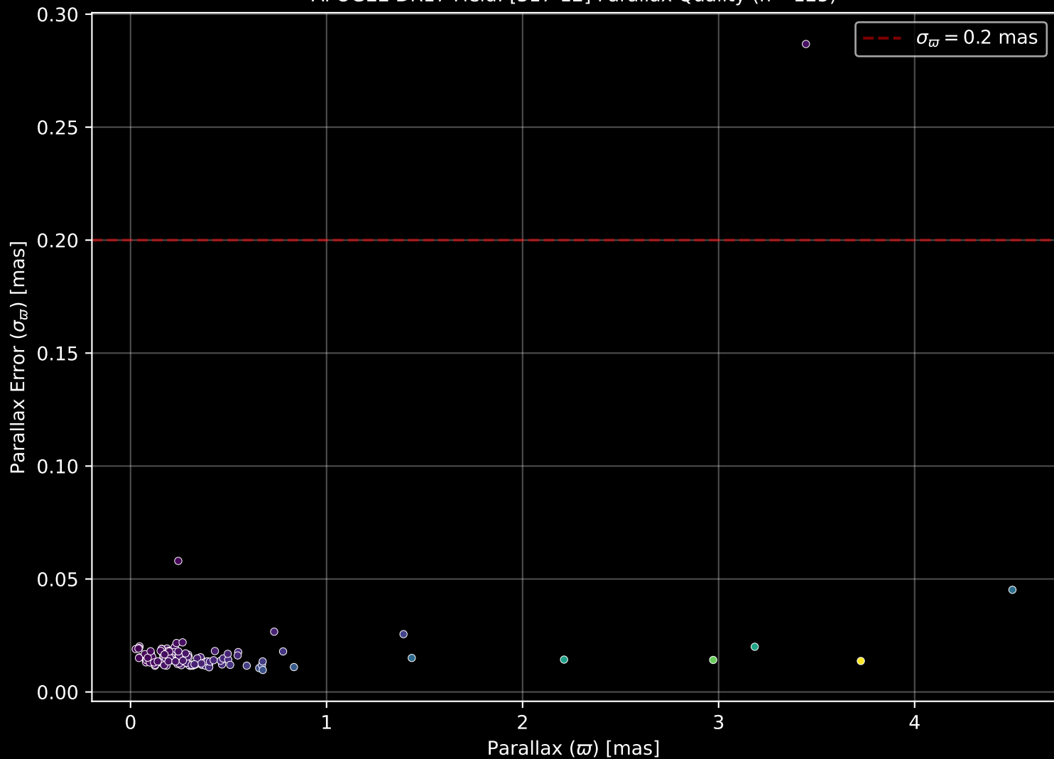
APOGEE DR17 Field: [317-12] Parallax Quality (n= 125)
