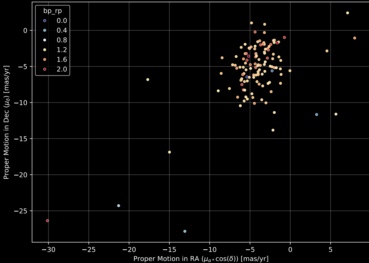
APOGEE DR17 Field: [317-12] Proper Motion Diagram (n= 125)
