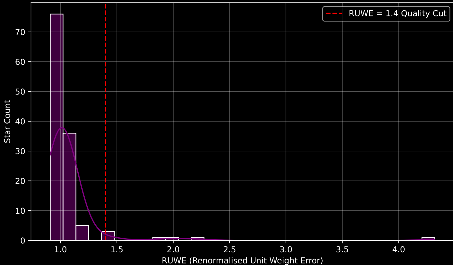
GAPOGEE DR17 Field [317-12] RUWE Distribution (n= 124)
