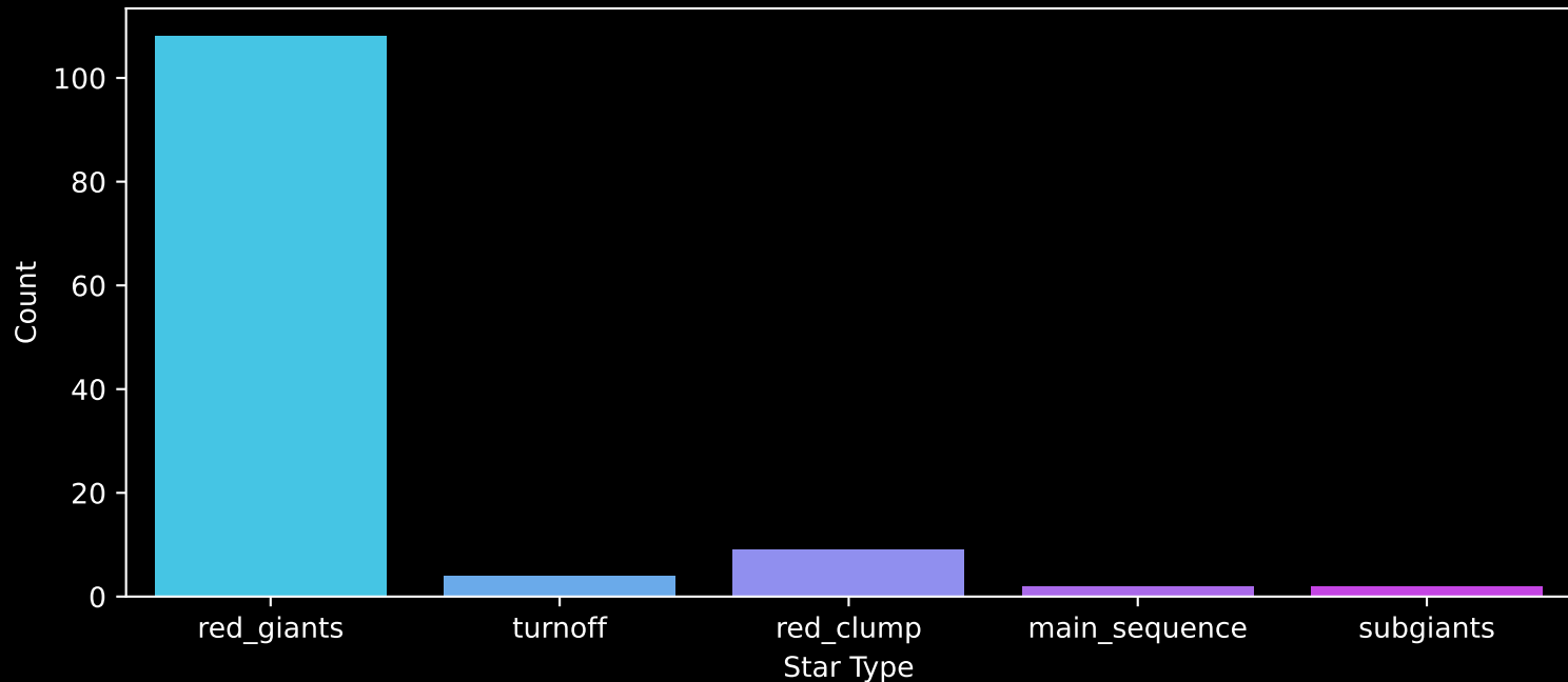
APOGEE DR17 Field: [317-12] Count plot of Star Type
