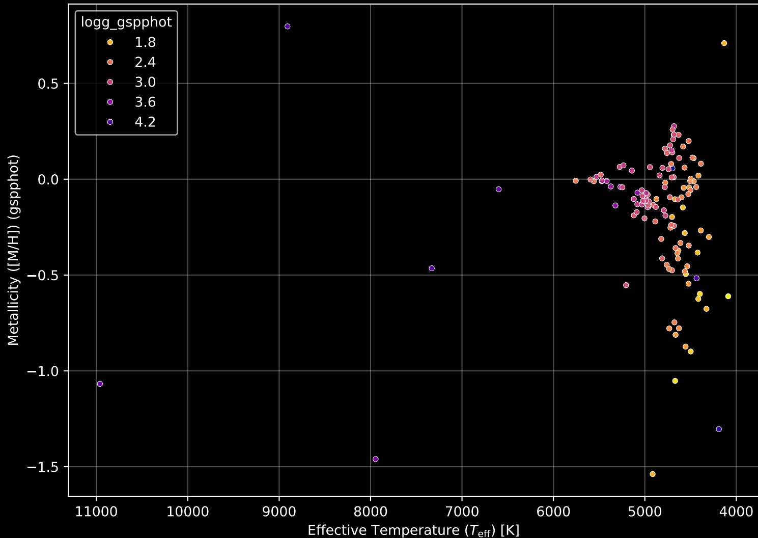
APOGEE DR17 Field: [317-12] Stellar Population Parameters (n= 125)
